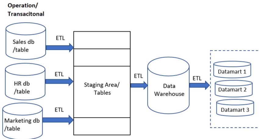
Figure 1.1: Data warehousing environment
